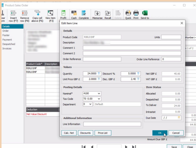
Sage Order Item Additional Details Edit Form
